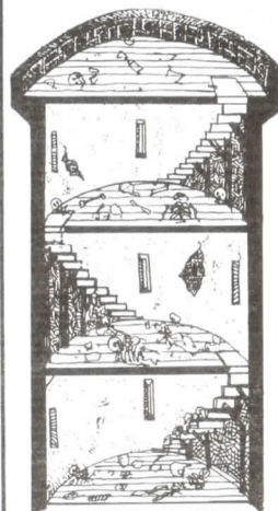
WATCHTOWER: cross-section
